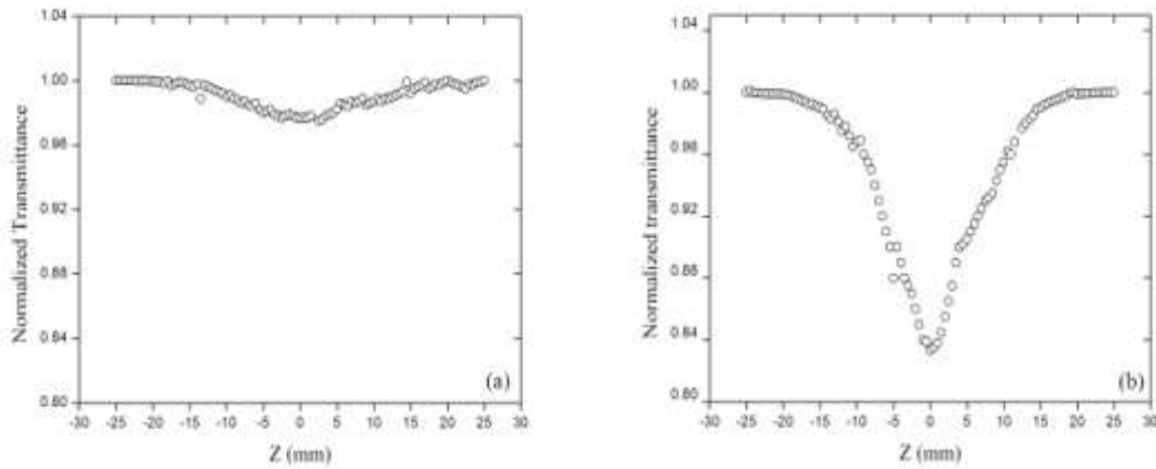
Fig.3. Open aperture Z -scan curve for (a) undoped (b) dye doped 1, 7, 7-Trimethylbicyclo [2.2.1] heptan-2-one.
