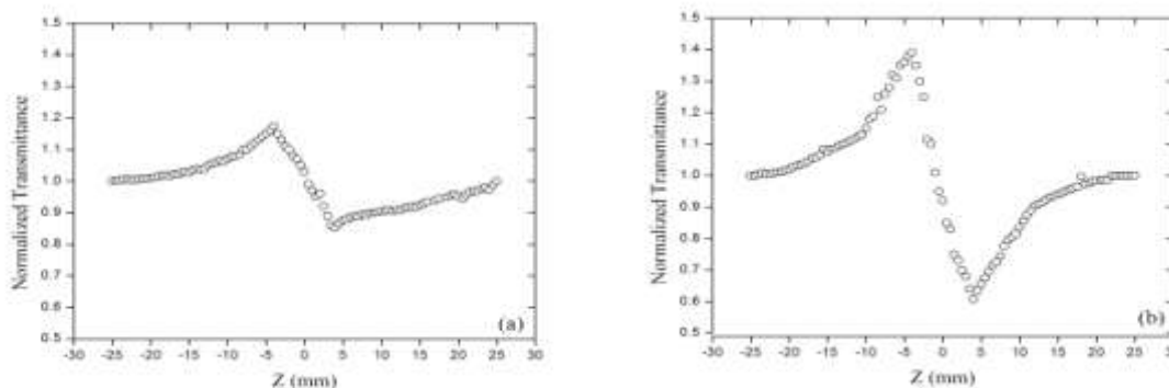
Fig.2. Pure nonlinear refraction curve for (a) undoped (b) dye doped 1, 7, 7-Trimethylbicyclo [2.2.1] heptan-2-one.
